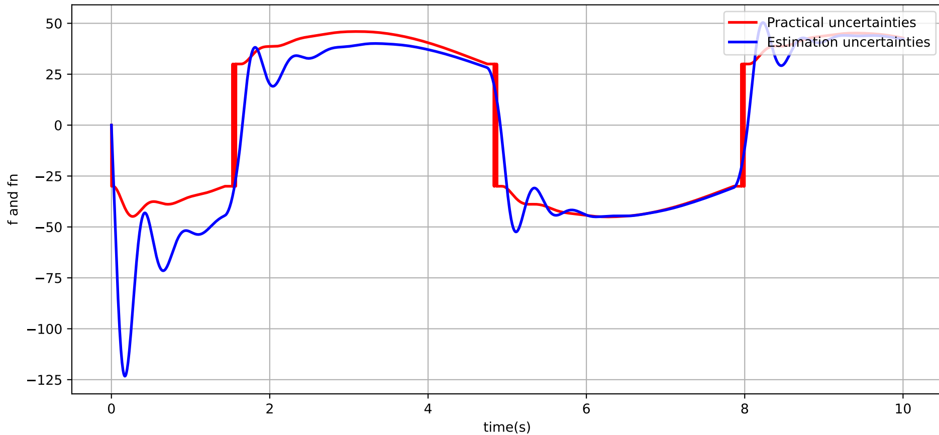
Disturbance Estimation Performance ( S=3 , S1=2 , m=19 )
